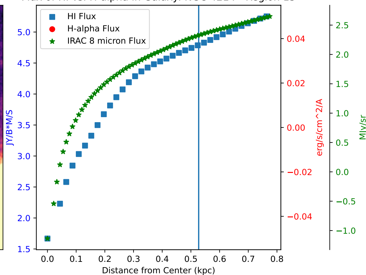
Flux of HI vs. H-alpha in Galaxy: NGC 4214 - Region 15
