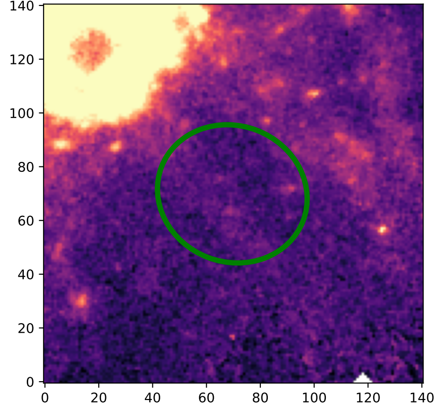
IRAC 8 micron - Classification: Diffuse
