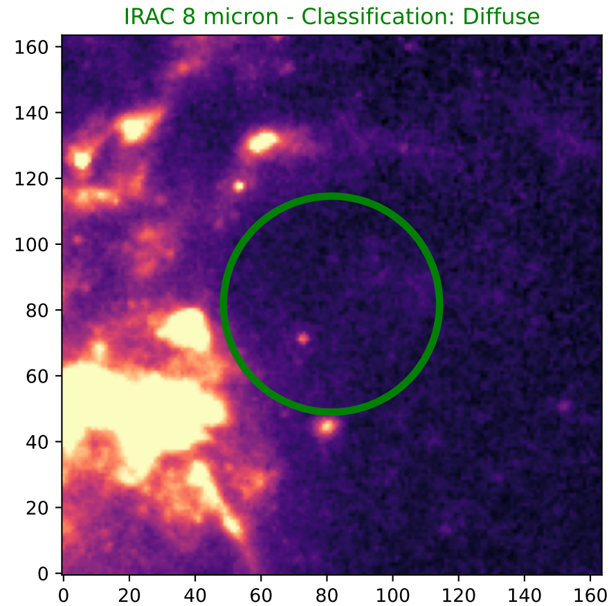
Flux of HI vs. H-alpha in Galaxy: NGC 4214 - Region 5
