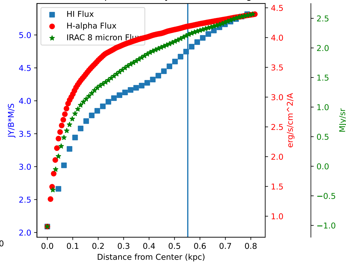
Flux of HI vs. H-alpha in Galaxy: NGC 4214 - Region 10
