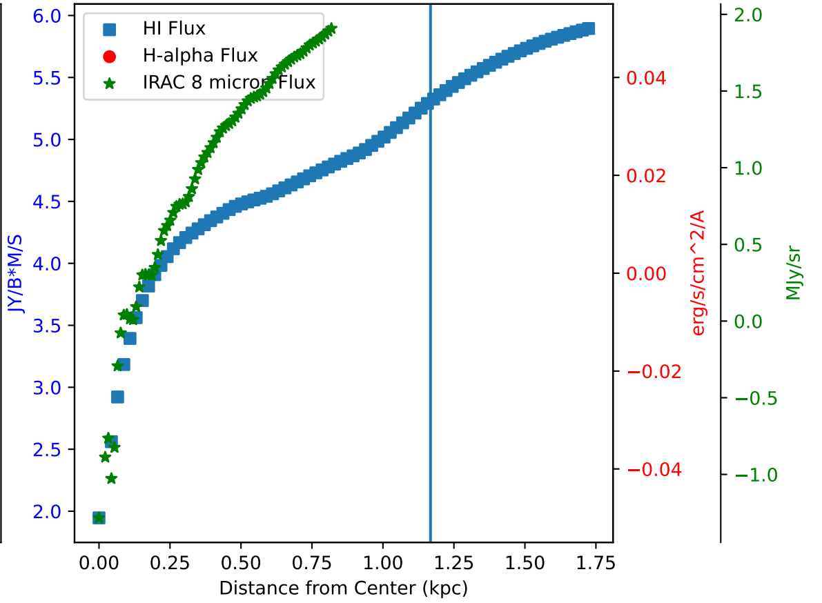
Flux of HI vs. H-alpha in Galaxy: NGC 4214 - Region 2
