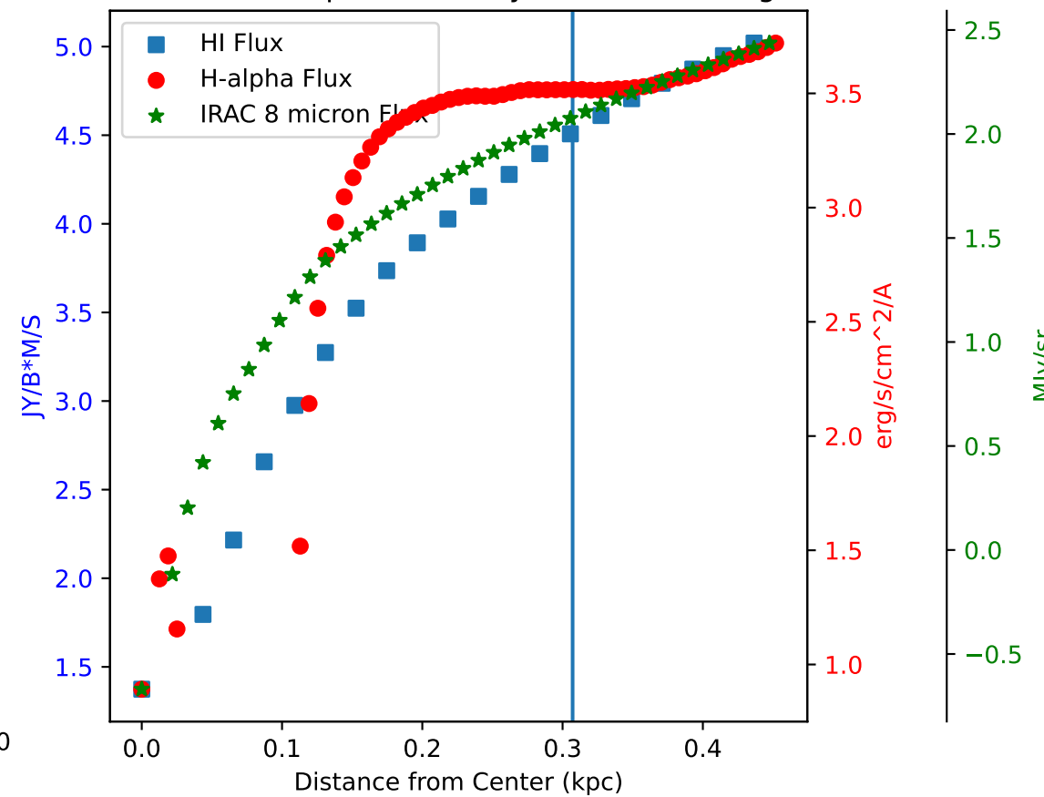
Flux of HI vs. H-alpha in Galaxy: NGC 4214 - Region 7
